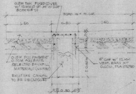
ROAD SECTION AT FIXED COVER BLOCK 29, 25, 26A, 26B, 27, 24
