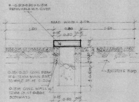
ROAD SECTION AT M.H. BLOCK 29, 25, 26A, 26B, 27, 24
