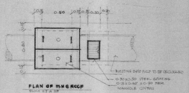
DETAIL M.H COVER AT CHS & RCP
